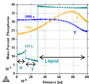
Microsegregation
